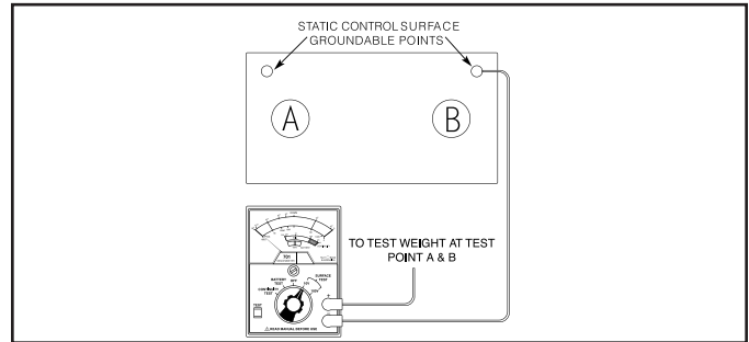
Figure 7. Material Evaluation Surface to Groundable Point Test.
