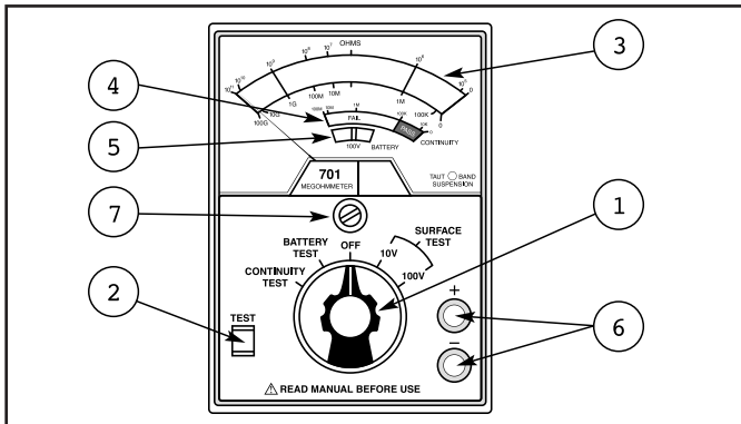
Figure 2. SCS 701 Analog Surface Resistance Megohmmeter Kit, controls, connectors and indicators.
