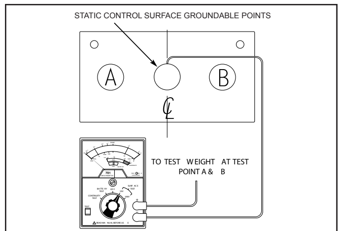
Figure 8. Material Evaluation Surface to Surface Test.
