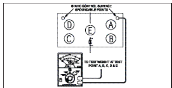
Figure 5. Qualification Tests of Installed Surfaces.
