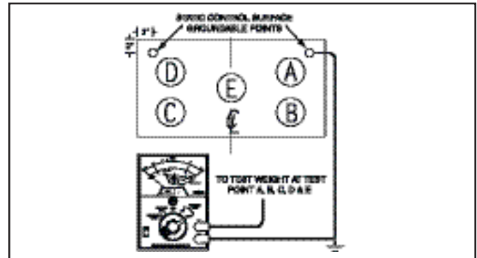
Figure 4. Periodic Preformance Tests of Installed Surfaces.
